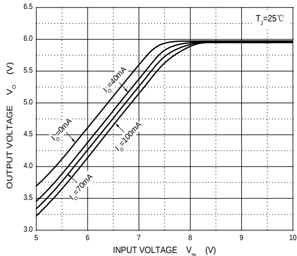
Dropout Characteristics
