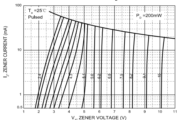
Temperature Coefficients
