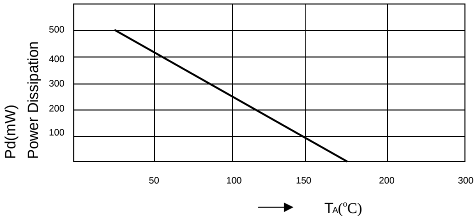
FIG.2- POWER ,TEMPERATURE DERATING CURVE
