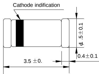
LL-34(SOD-80) Dimensions in millimeters
