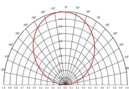
◆ Directive Characteristics Red(y)
