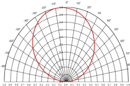
◆ Directive Characteristics Red(x)
