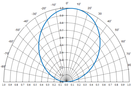
◆ Directive Characteristics Blue(x)
