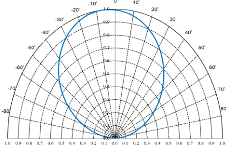
◆ Directive Characteristics Blue(y)
