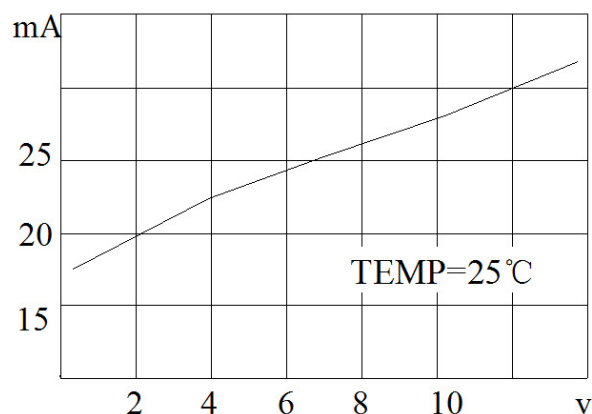
VOLTAGE-CURRENT CONSUMPTION
