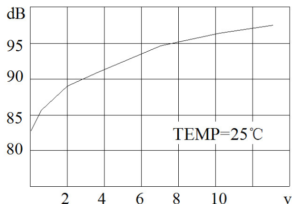
VOLTAGE-SOUND PRESSURE LEVEL
