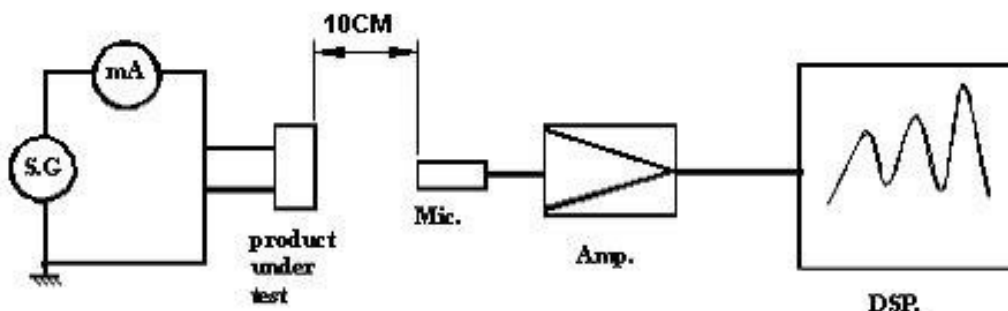
Fig.1 Measuring circuit:
