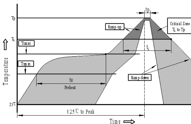
Fig. 6 Soldering condition:
