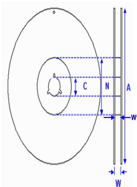
Fig. 9.3 The dimension of reel
