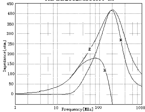
HDGB2012M601HT-LF
