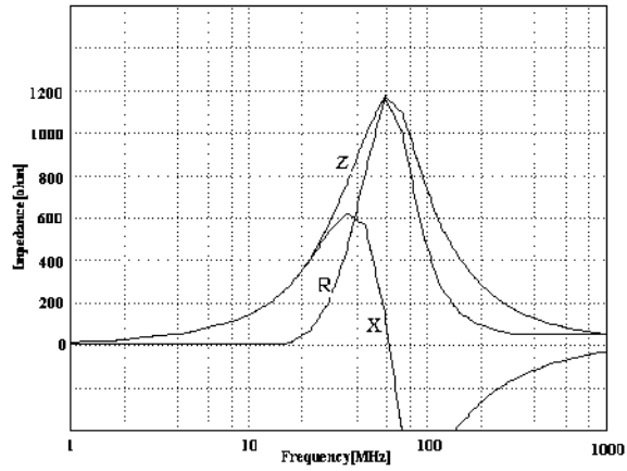
HDGB3216M122HT-LF
