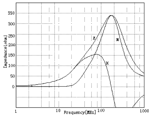
HDGB3216M301HT-LF
