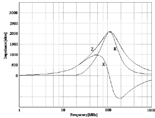
HDGB1608M182HT-LF
