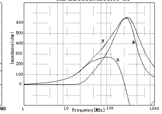
HDGB1608M501HT-LF
