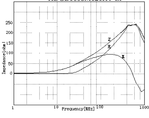
HDGB1608M301HT-LF
