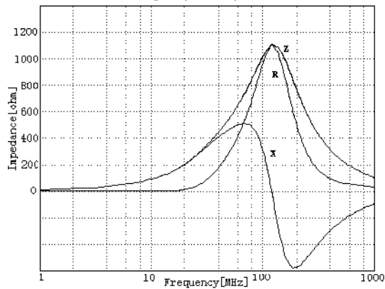
HDGB2012M102HT-LF
