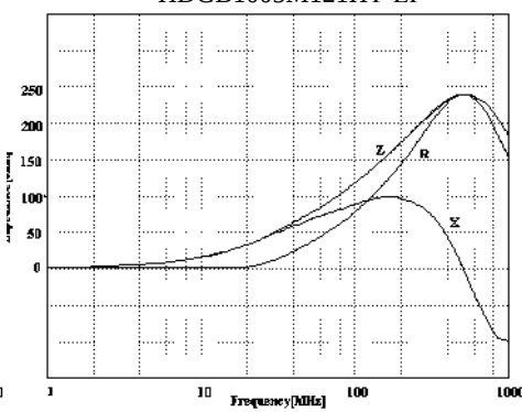
HDGB1005M501HT-LF
