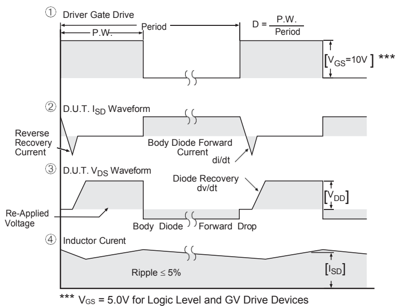
Fig 13. For P-Channel HEXFETS
