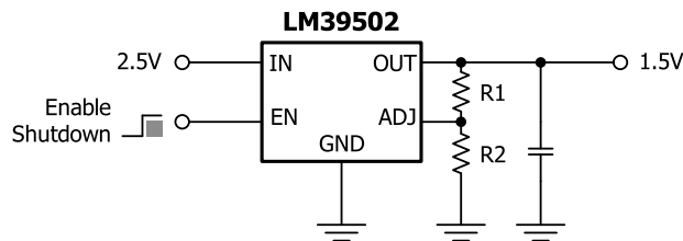
1.5V / 5A Adjustable Regulator
