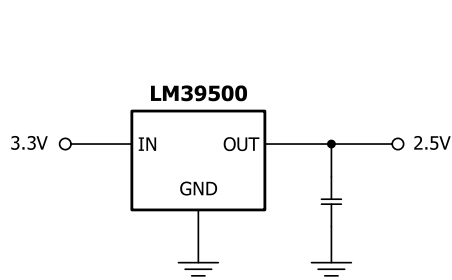
2.5V / 5A Regulator
