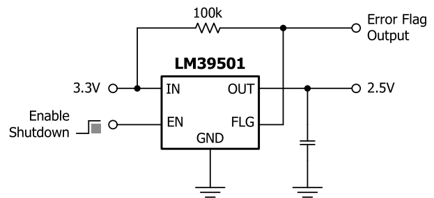
2.5V / 5A Regulator with Error Flag
