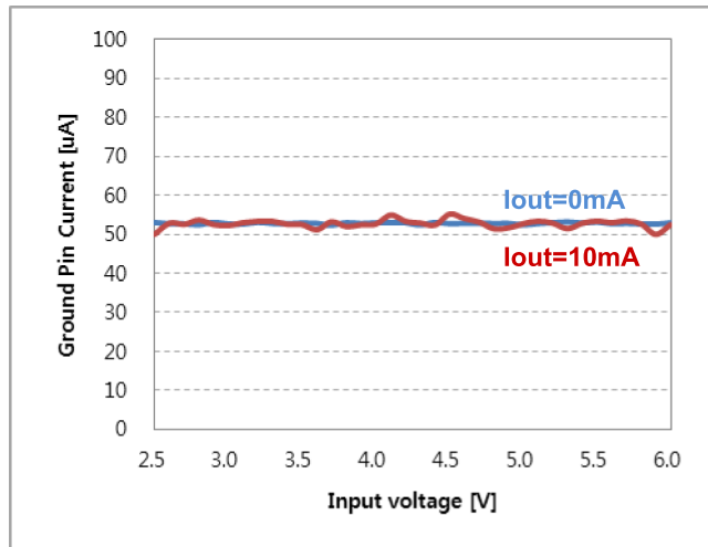
Ground Currnet @ Iout=0A / 10mA (Cin=10uF, Cout=10uF, R2=36KΩ, R1=35KΩ)
