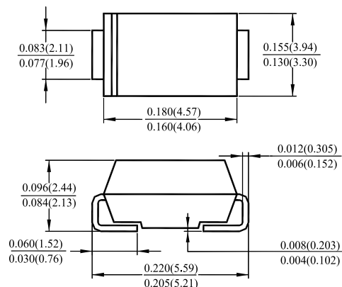
Dimensions in inches and (millimeters) DO-214AA (SMB)
