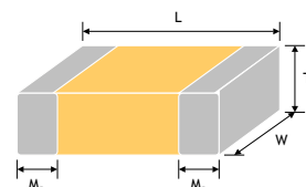
Fig. 5.1 The outline of MLCC
