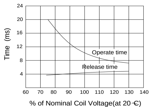
Operate time/Release time
