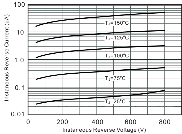
Fig.2 Typical Instantaneous Reverse Characteristics
