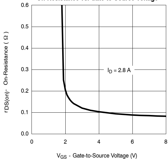
On-Resistance vs. Gate-to-Source Voltage
