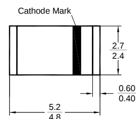
Plastic case MELF (DO-213AB) Dimensions in mm
