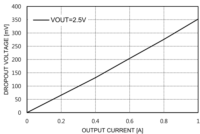
Dropout Voltage
