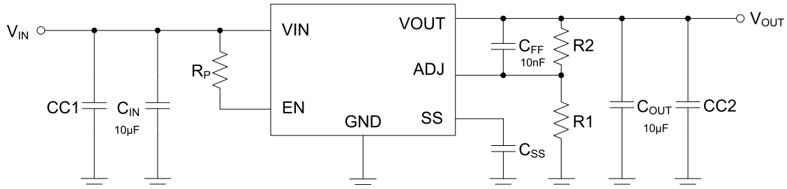
Fig. 2. Application with Feed-Forward Capacitor, CFF
