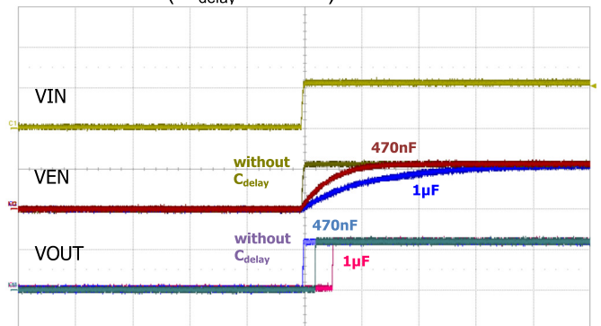
VOUT = 1.2V ( C_{delay} : varied )
