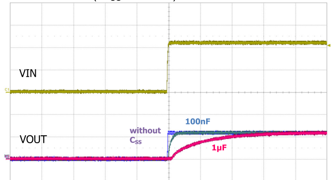
VOUT = 1.2V ( C_{SS} : varied )
