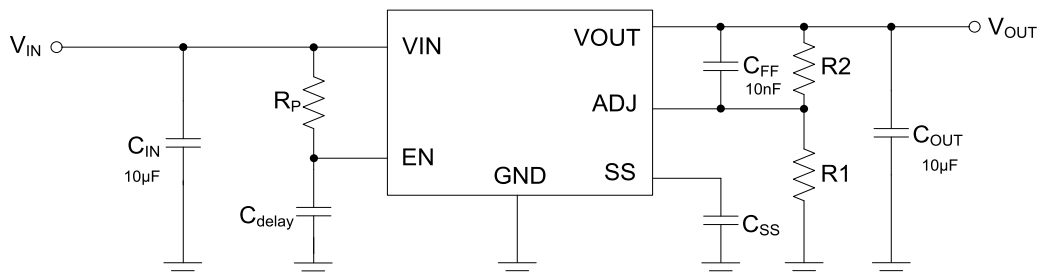
Fig. 3. Application with Delayed Start-Up
