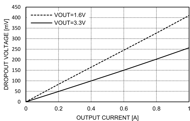
Dropout Voltage
