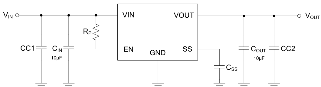
Fig. 1. Application with Decoupling Capacitor, CC1 & CC2
