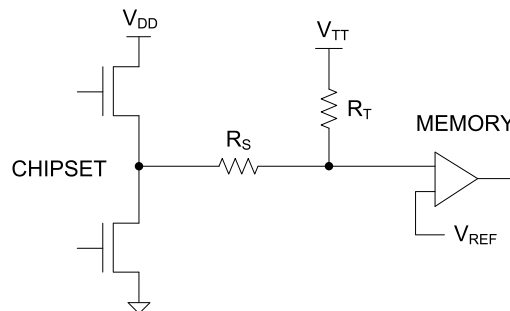
Fig. 1. SSTL-Termination Scheme
