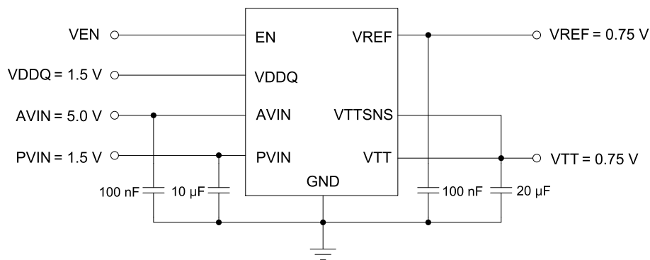
Fig. 5. HSTL Application
