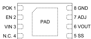
DFN2X3-8L (Top view)
