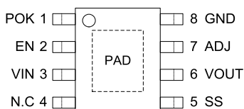
SOP8-PP
