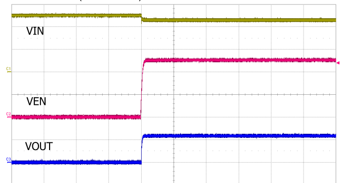
VIN : 1.0V/div, VEN : 1.0V/div, VOUT : 1.0V/div, Time : 5ms/div Start Up by External VEN @ Iout=3A
