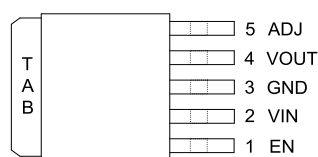
TO-252-5L
