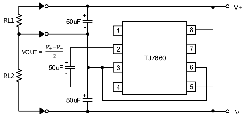
Figure 21. Splitting a Supply in Half
