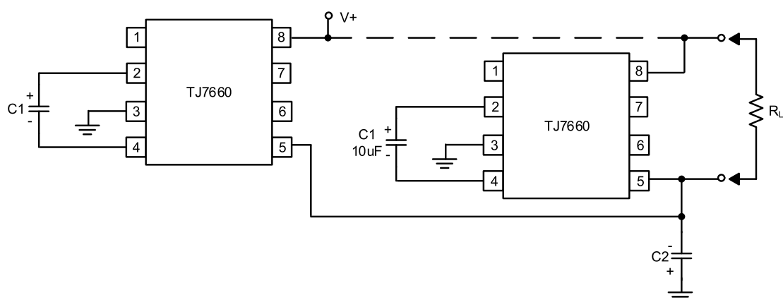
Figure 15. Paralleling Devices
