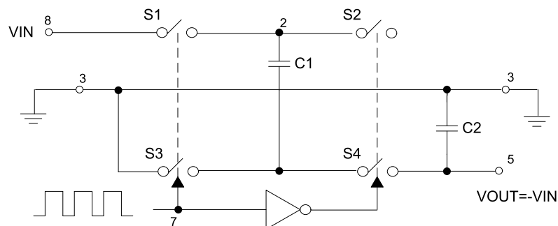
Figure 12. Idealized Negative Voltage Converter
