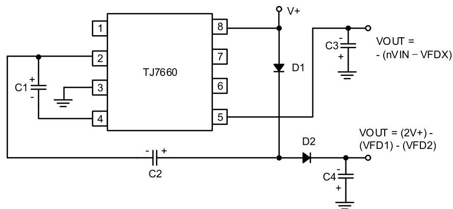
Figure 20. Combined Negative Voltage Converter and Positive Doubler
