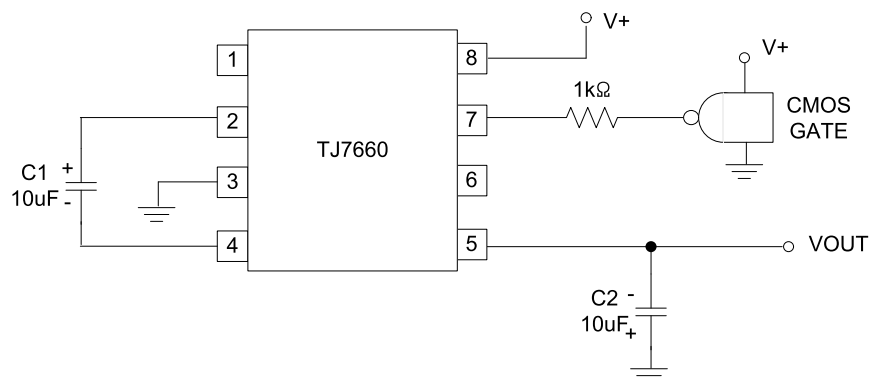
Figure 17. External Clocking
