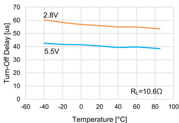
Turn Off Delay Time vs. Temperature
