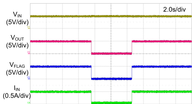
Thermal Shutdown
