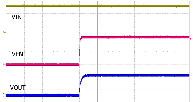
Start Up by External VEN @ Iout=300mA
