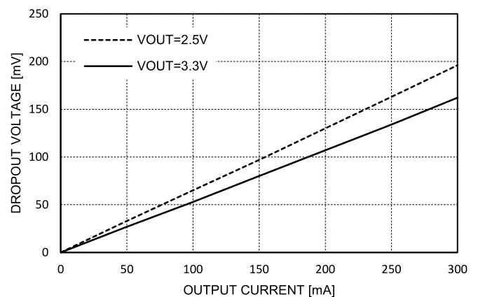
Dropout Voltage
