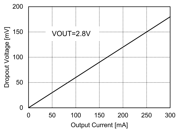
Dropout Voltage
