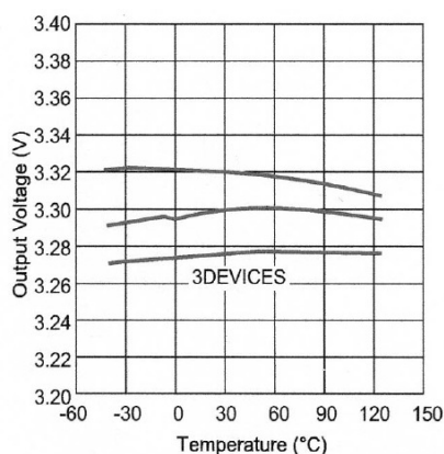
3.3V Output Voltage vs. Temperature
