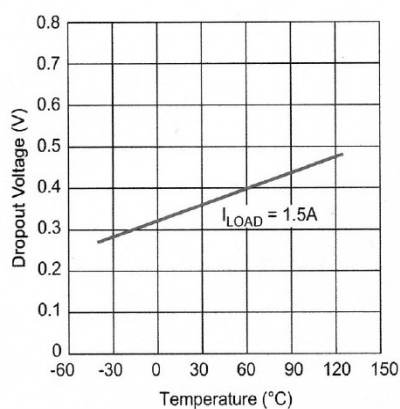
Dropout Voltage vs. Temperature
