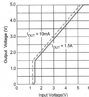
5.0V Dropout Characteristics
