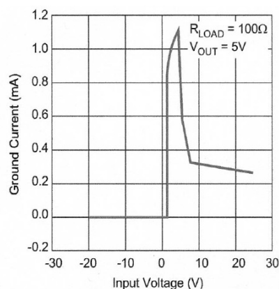
Ground Current vs. Input Voltage
