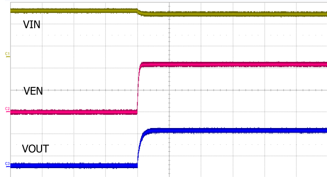
Start Up by External VEN @ Iout=2A
