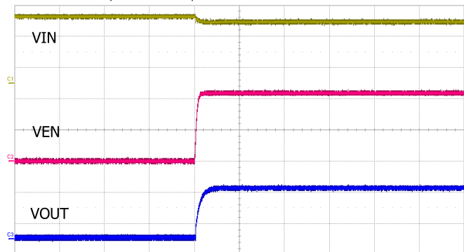
Start Up by External VEN @ Iout=3A
