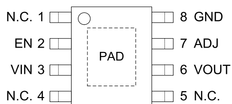
SOP8-PP
