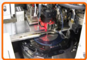
Dicing
